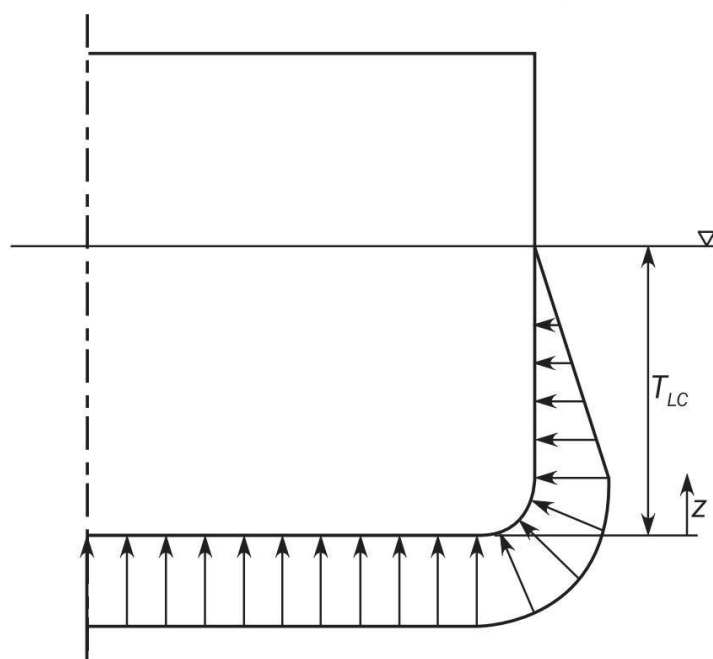
Figure 2.7.5 Schematic diagram of hydrostatic pressure,
