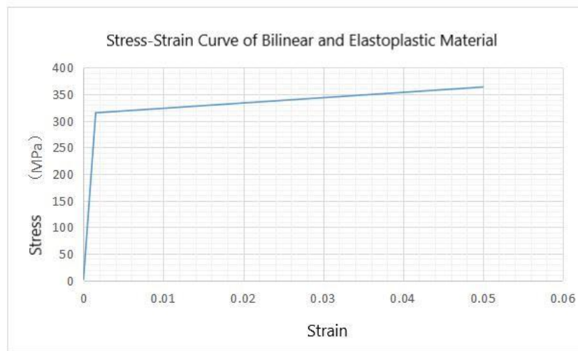
Figure 2.5.1 Schematic diagram of stress-strain curve of material
