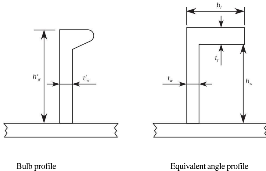
Figure 2.1. 4 Equivalent dimension of bulb profile
