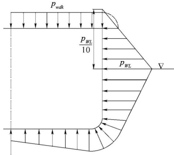
Figure 2.7.6 Schematic diagram of external seawater dynamic pressure
